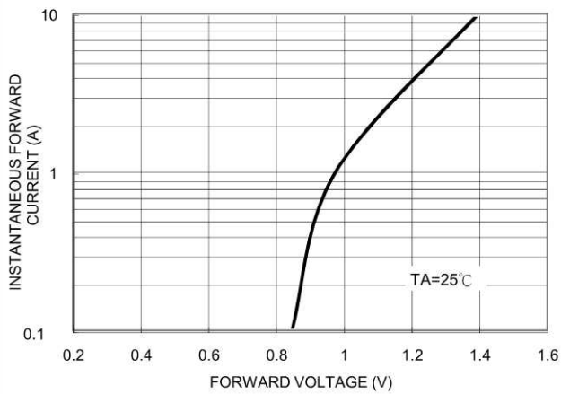
FIG. 5 TYPICAL FORWARD CHARACTERISTICS PER LEG
